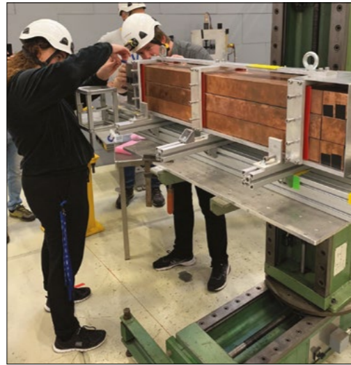
Saturation specific ALICE's new high-granularity forward calorimeter is designed to study gluon saturation.
