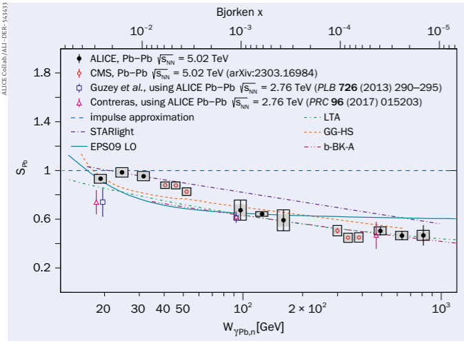
Nuclear shadowing The nuclear suppression factor for lead relative to protons ( S_{pA} ) as a function of energy and Bjorken x . No model can yet describe saturation and shadowing over the measured kinematic domain.
