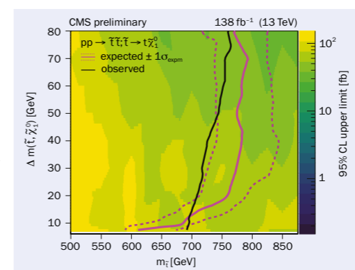
Fig. 1. Limits on stop pair production with decays through top quarks and LSPs. The colour scale shows 95% CL upper limits on the product of the cross-section and branching fractions as a function of stop mass and stop-LSP mass difference. The expected (magenta line) and observed (black line) lower mass limits are indicated assuming 100% branching fractions.
