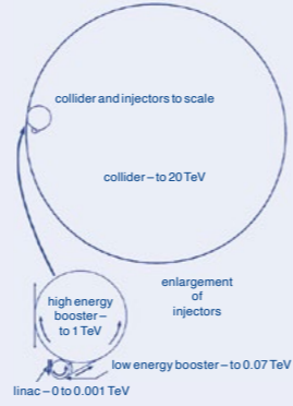
A possible SSC injection scheme.
