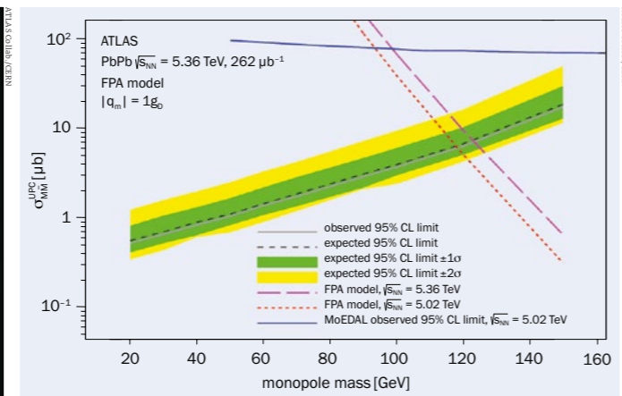
Fig. 2. 95% confidence upper limits on the monopole pair-production cross-section in PbPb ultraperipheral collisions at 5.36 TeV. The limits are compared with model predictions and limits from the MoEDAL experiment.
